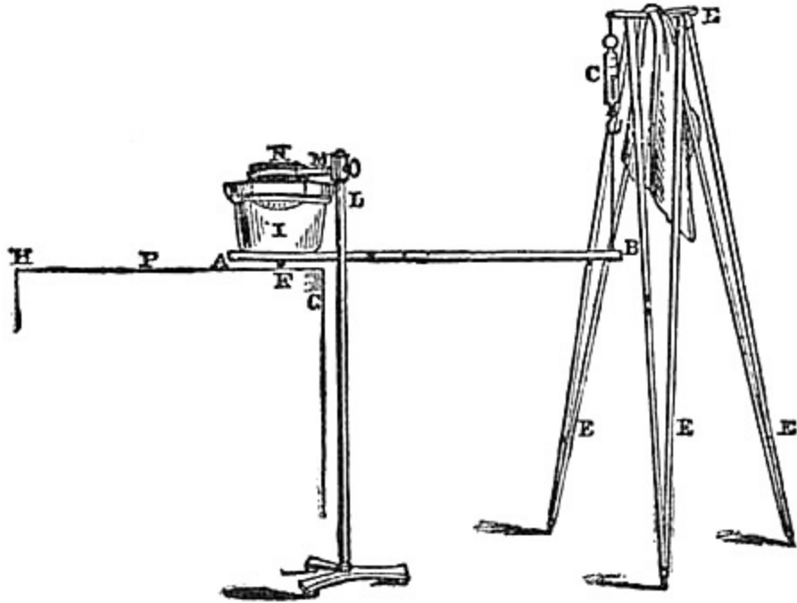
FIG. 9. CROOKES' APPARATUS.
