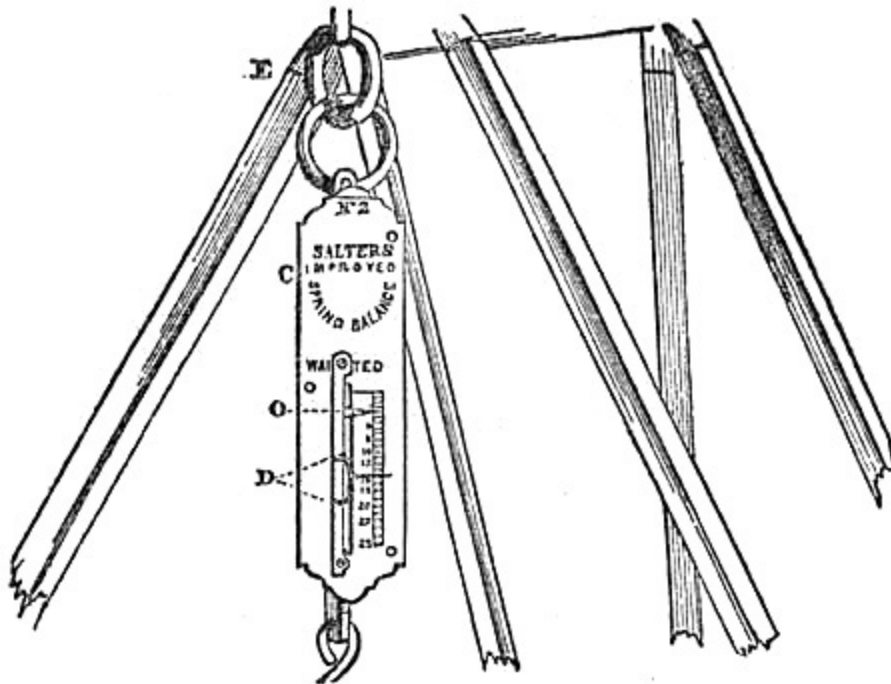
FIG. 10. CROOKES' APPARATUS.
